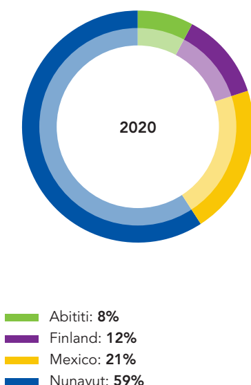
Figure 5. Proportion of Total GHG Emissions (Scope 1 and 2) by Region
